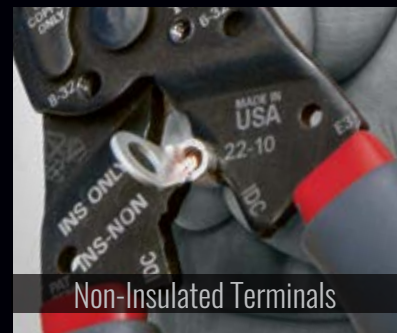
B Connectors
